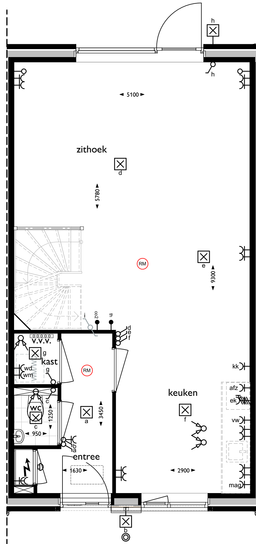
00 begane grond
