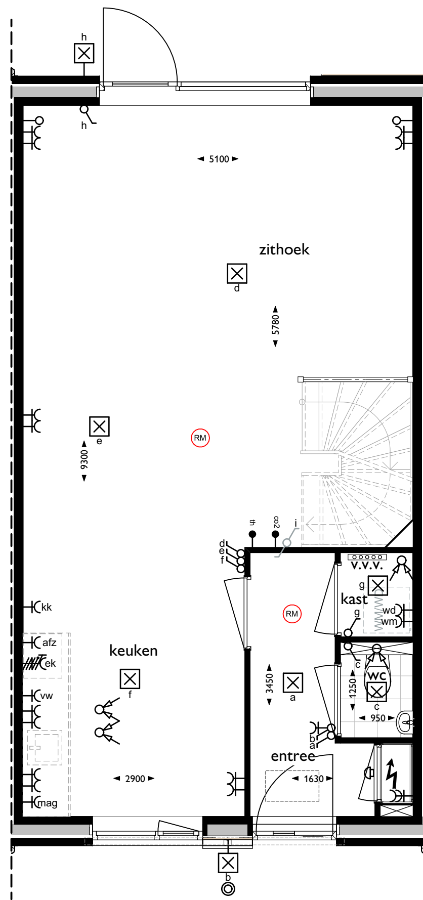
00 begane grond
